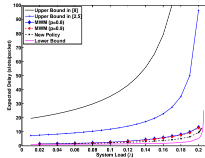
Figure 3: Simulation results for Tree Topology
