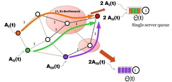
Figure 1: Reduction technique to derive a fundamental lower bound on the expected delay of a wireless-network
