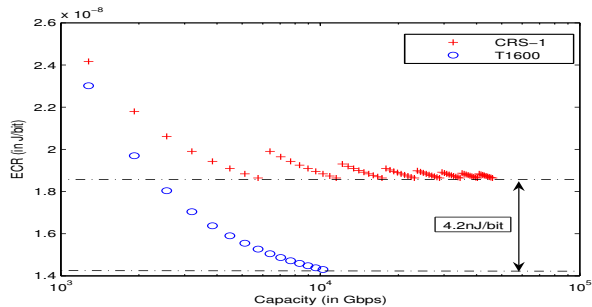
(b) Energy per bit Vs Capacity
