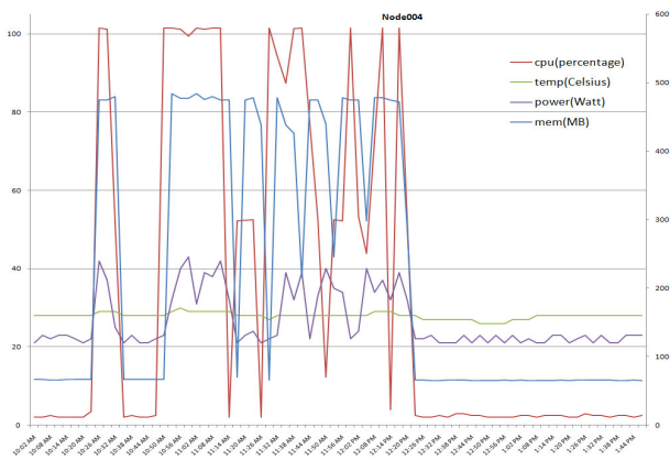
Figure 1. Resource and Energy Consumption. A typical example of CPU, memory, temperature and power usage of a server node.
