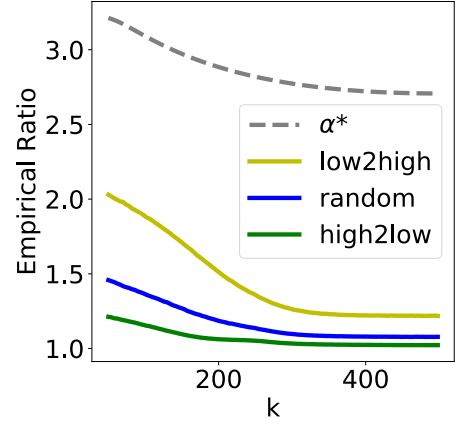
Figure 2: Performance of \text{TP}_{\lambda^*} under different types of arrival instances. Other than \alpha^* , each curve shows the empirical ratio of \text{TP}_{\lambda^*} over 1000 arrival instances sampled by their corresponding types.
